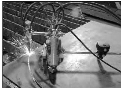
CIRCULAR CUTTING ATTACHMENT Radius 50-550mm (2-22in): ZS31858
